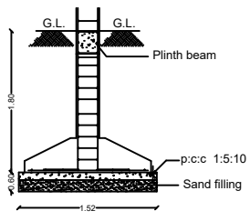
FOUNDATION DETAILS
