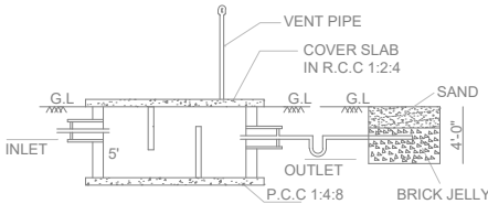
SECTION-AB
