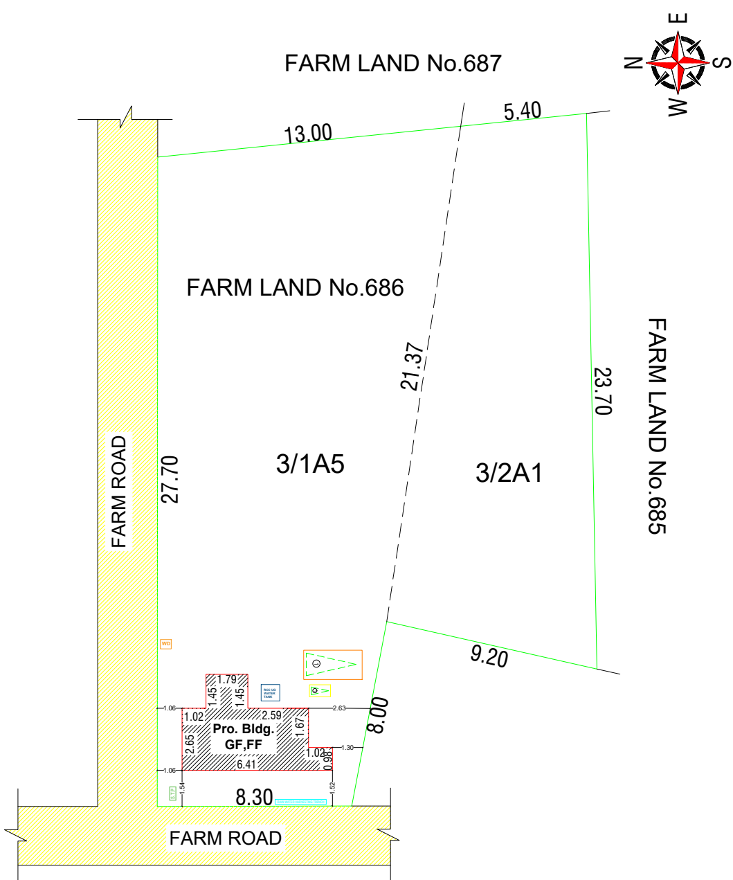
SITE PLAN
