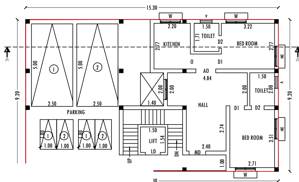
FLOOR PLAN
