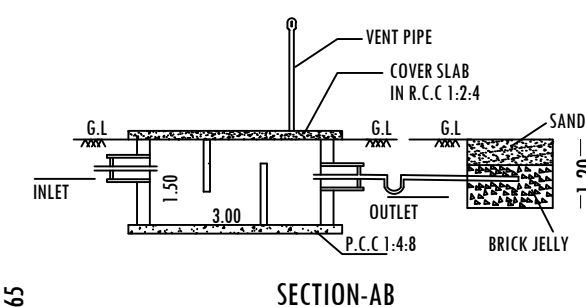
SECTION-AB
