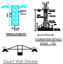
Dwarf Wall Details
