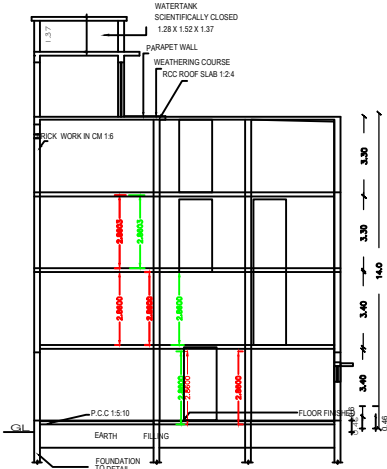
SECTION "A-B"
