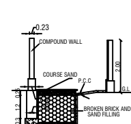
PLINTH BOUNDARY PERCOLATION PIT
