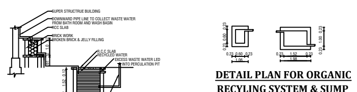
DETAIL PLAN FOR ORGANIC RECYCLING SYSTEM & SUMP
