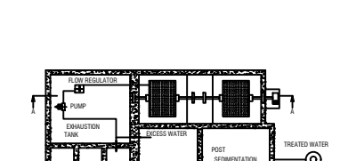
SEWAGE TREATMENT PLANT (STP)
