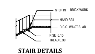
STAIR DETAILS
