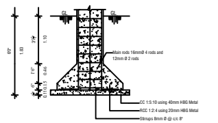
DETAIL
