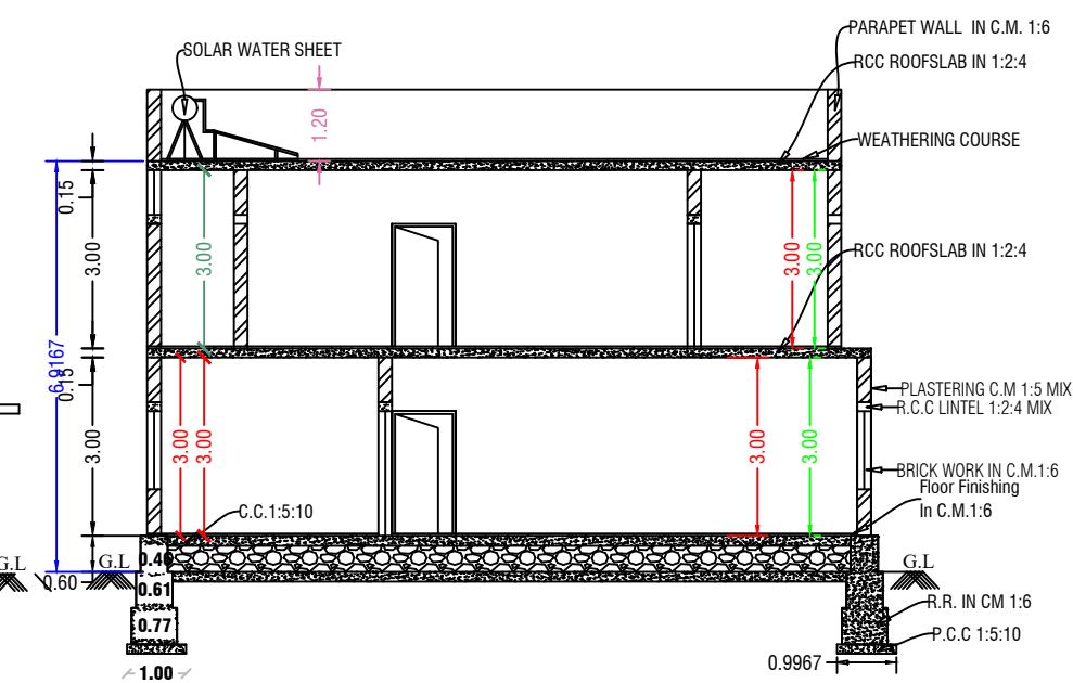
Section On-'AB'
