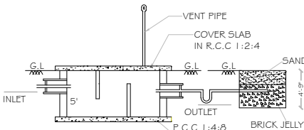
SECTION-AB
