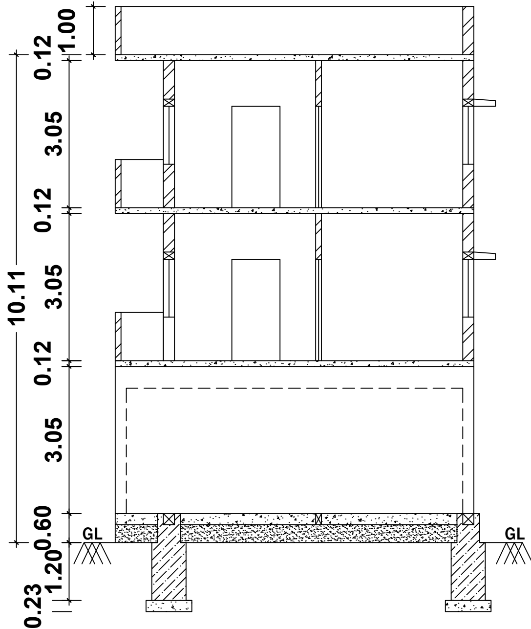
SECTION "A-B"
