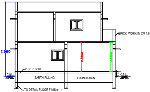
SECTION "A-B"
