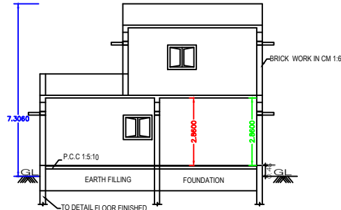
SECTION "A-B"
