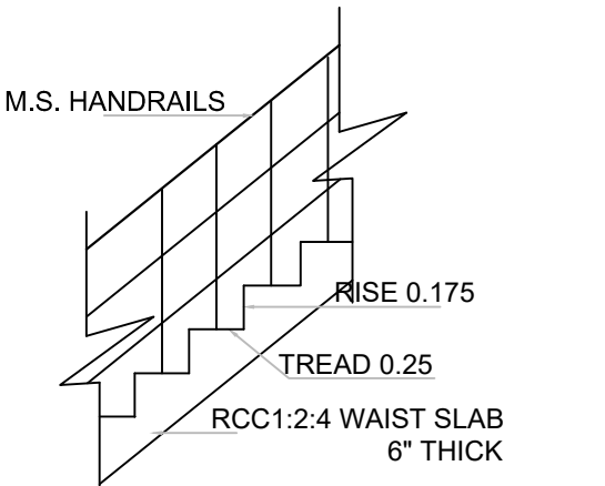
STAIRCASE DETAILS
