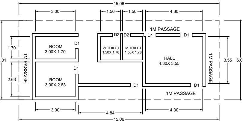
FLOOR PLAN
