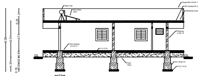
SECTION AT 'AA'
