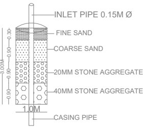
DETAILS OF RAIN WATER H/
