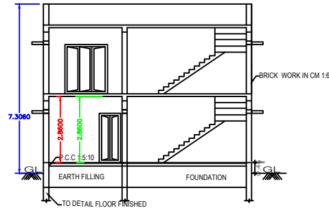
SECTION "A-B"
