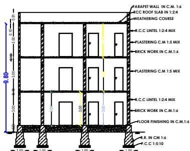
SECTION ON-"AB"
