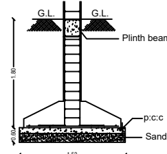
FOUNDATION DETAILS
