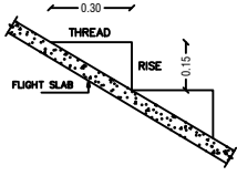
STAIRCASE DETAILS
