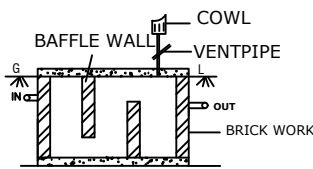
SECTION ON - XY
