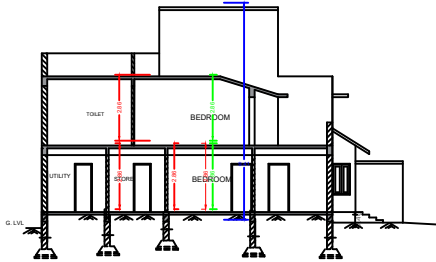
SECTION "A-B"
