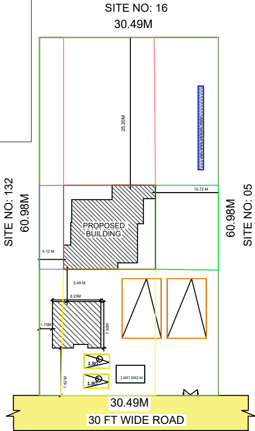
SITE PLAN
