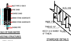
DETAILS OF RAIN WATER HARVESTING STRUCTURES
