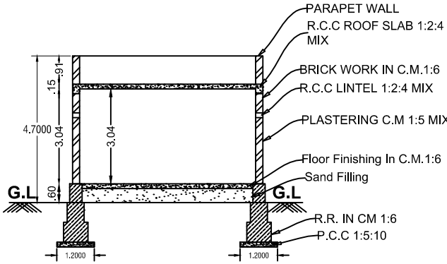
SECTION ON-"AB"
