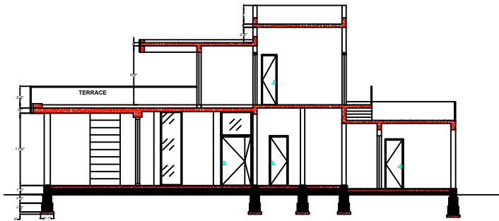
SECTION CC
