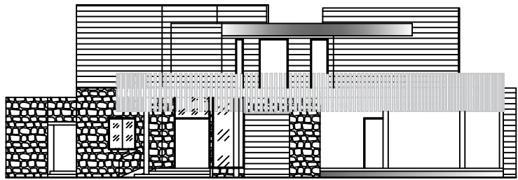
ELEVATION AA
