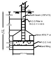
FOUNDATION DETAILS
