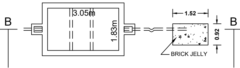
SEPTIC TANK DISPERSION TRENCH PLAN
