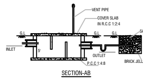
SECTION-AB
