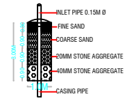
DETAILS OF RAIN WATER HARVESTING STRUCTURES
