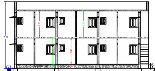
SECTION "A-B"
