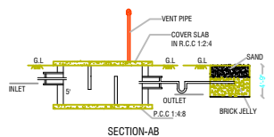
SECTION-A-B
