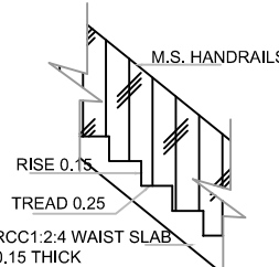
STAIRCASE DETAILS SCALE- 1:20
