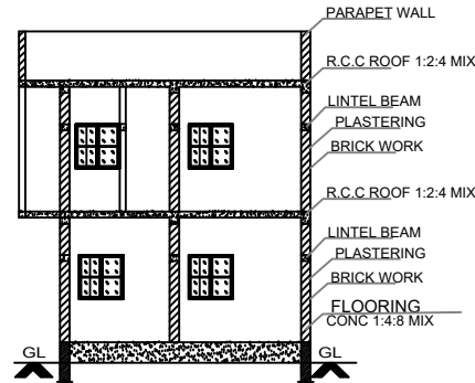
SECTION: A-B
