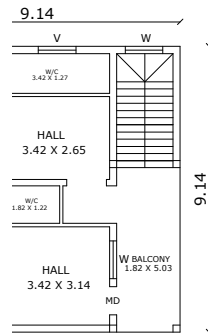
FLOOR PLAN
