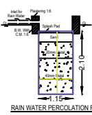
RAIN WATER PERCOLATION PIT
