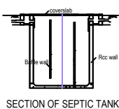
SECTION OF SEPTIC TANK
