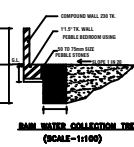
RAIN WATER COLLECTION TANK (SCALE-1:1000)
