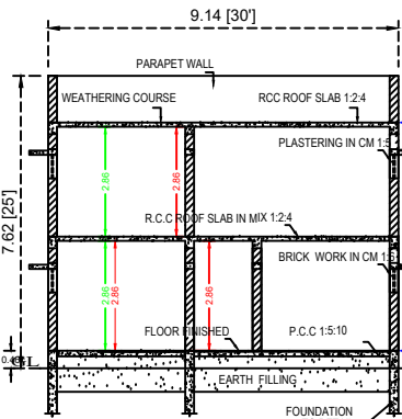
SECTION "A-B"
