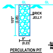
PERCOLATION PIT
