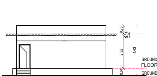
SERVANT QUARTERS NORTH SIDE ELEVATION
