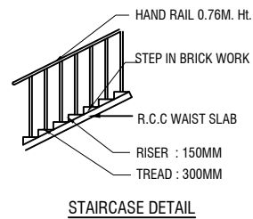
STAIRCASE DETAIL
