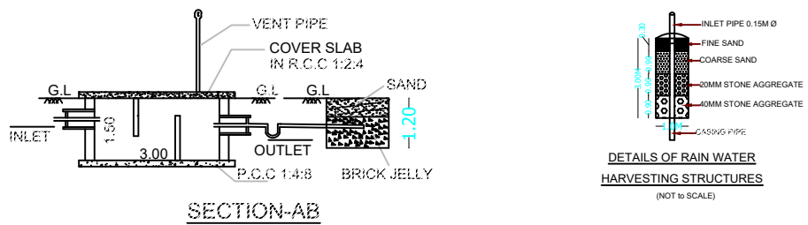
SECTION-AB
