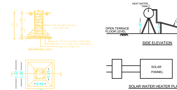
SOLAR WATER HEATER PLAN
