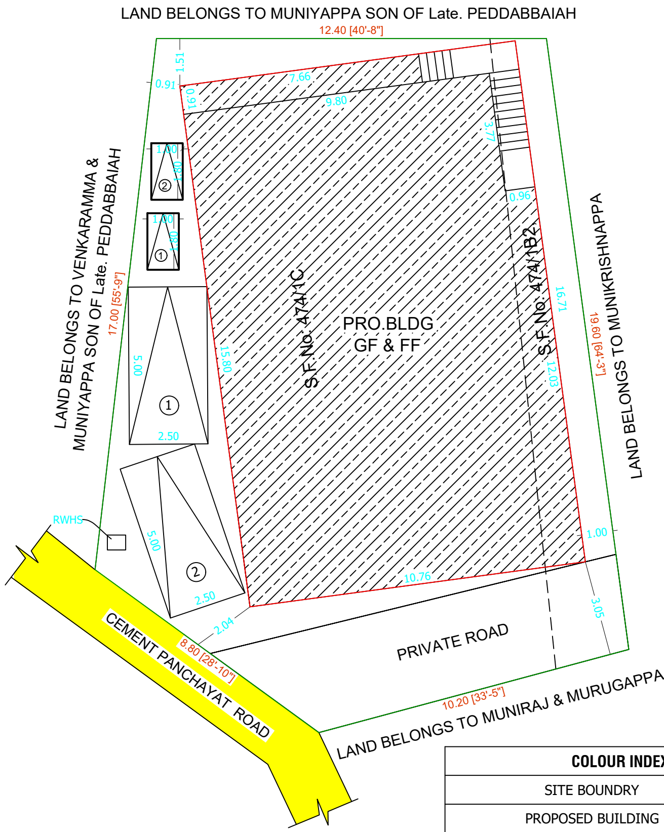
SITE PLAN
