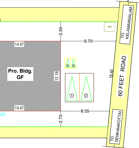
SEPTIC TANK & DISPERSION TRENCH DETAILS SCALE-1:100
