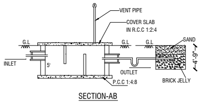
SECTION-AB
