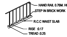
STAIR CASE DETAIL
