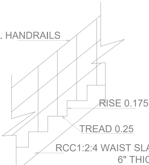
STAIRCASE DETAILS
