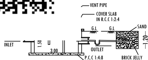
SECTION-AB
