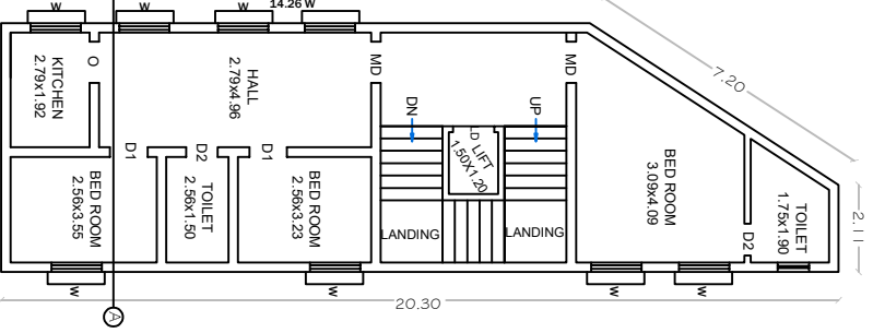
THIRD FLOOR PLAN
