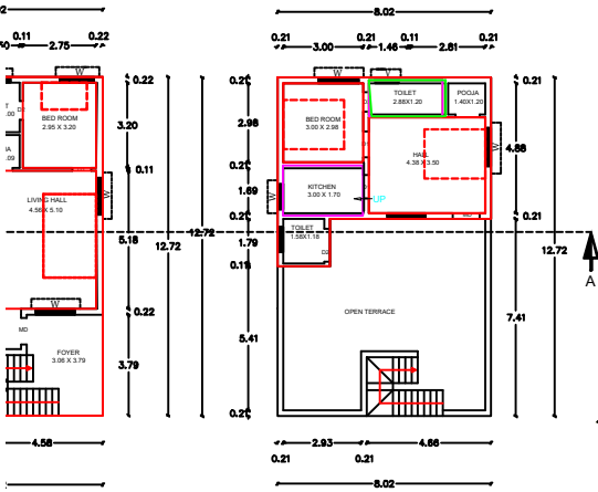
F FLOOR PLAN
