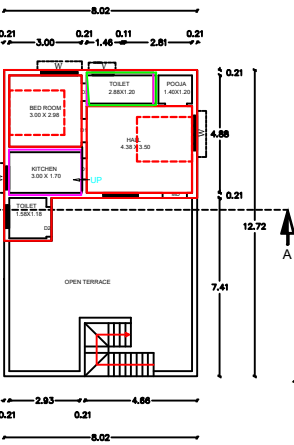
PRO.SECOND FLOOR PLAN
