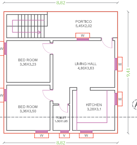
PRO. SECOND FLOOR PLAN.
