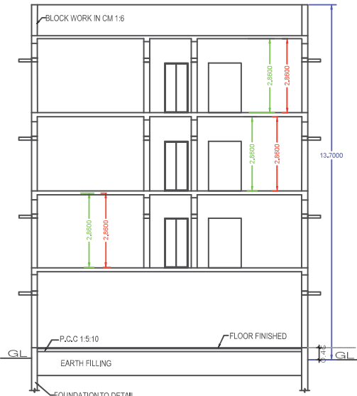
SECTION "A-B"
