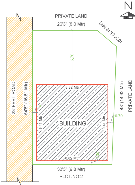
SITE PLAN
