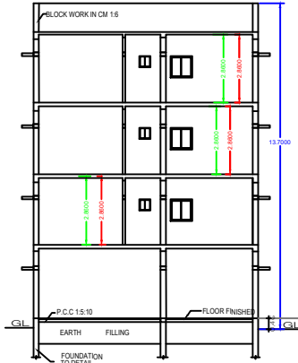
SECTION "A-B"
