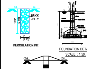
Dwarf Wall Details
