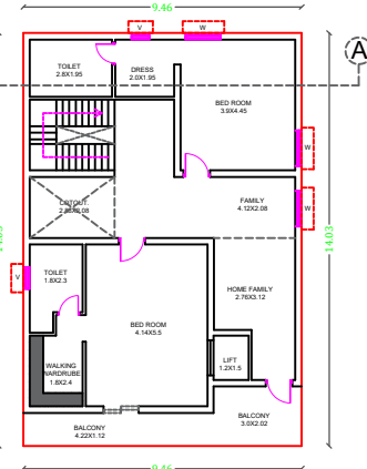
PRO. SECOND FLOOR PLAN.
