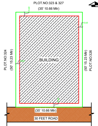
SITE PLAN
