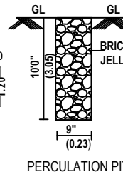
PERCOLATION PIT
