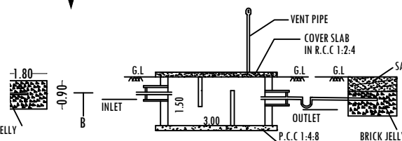
SECTION-AB
