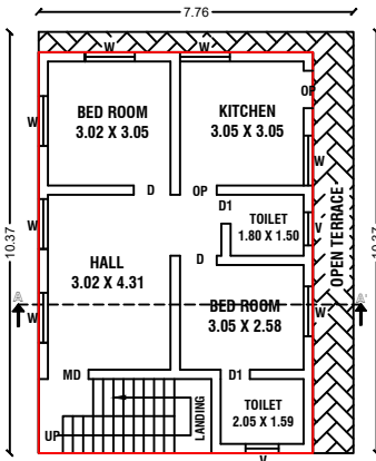
PROPOSED SECOND FLOOR PLAN
