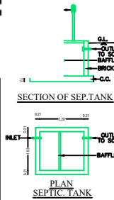
PLAN SEPTIC TANK
