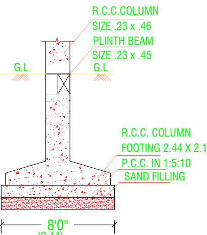
FOUNDATION DETAIL (DETAILS B)
