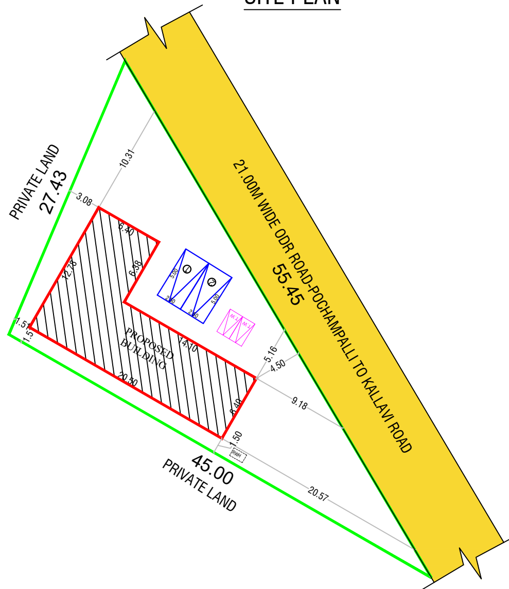
SITE PLAN
