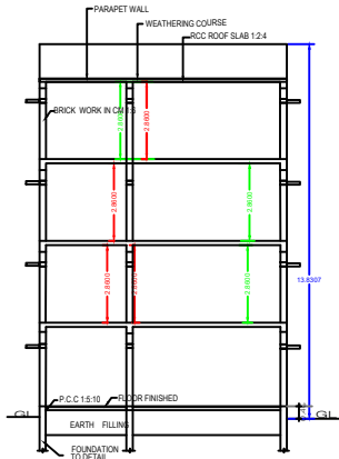
SECTION "A-B"
