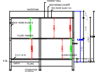
SECTION "A-B"
