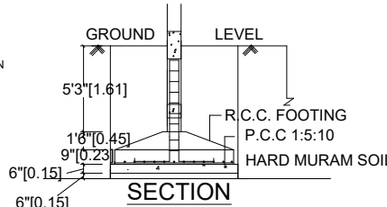
FOUNDATION DETAILS
