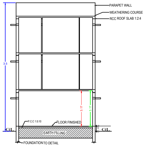
SECTION "A-B"
