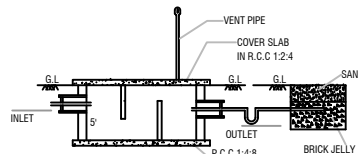
SECTION-A-B
