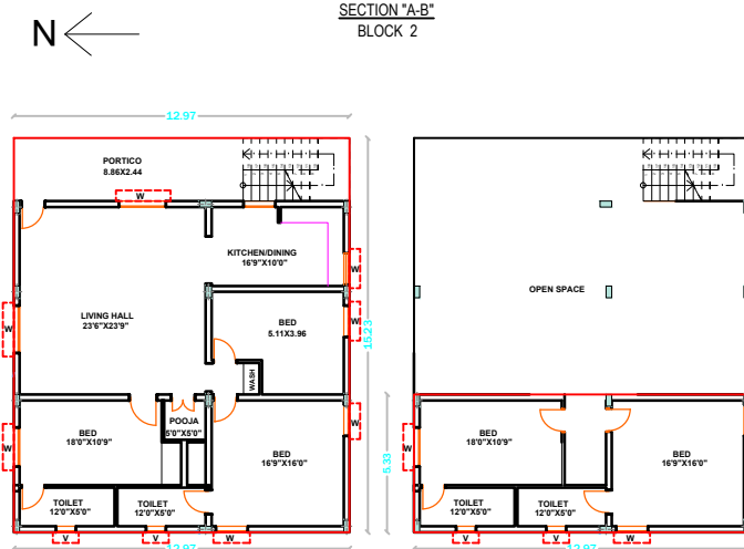
BLOCK - 2 EXI.GROUND FLOOR PLAN
