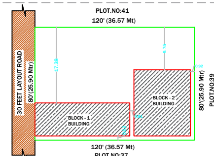
SITE PLAN SCALE:1:100
