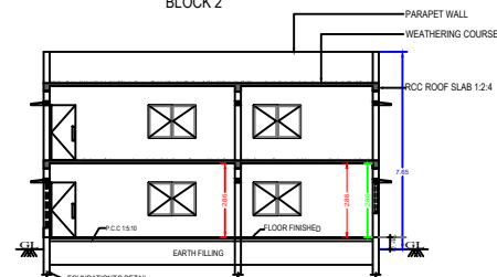
SECTION "A-B" BLOCK 2
