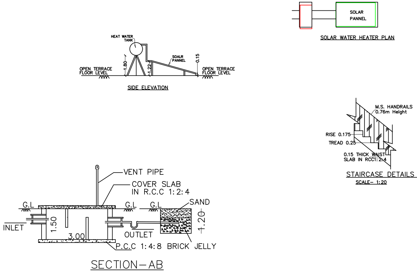
SECTION-AB
