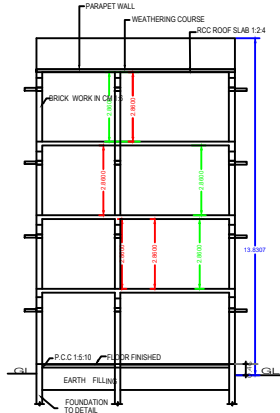
SECTION "A-B"
