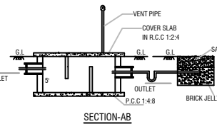
SECTION-AB
