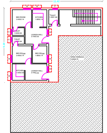
PRO.FIRST FLOOR PLAN. (RESIDENTIAL)
